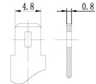
Terminal T1
